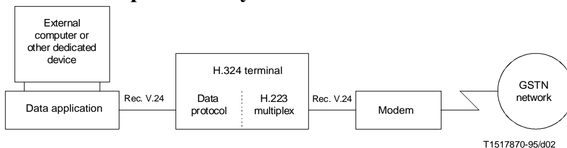
FIGURE 2/H.324
