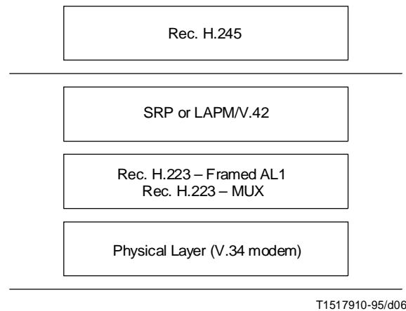
FIGURE A.1/H.324
