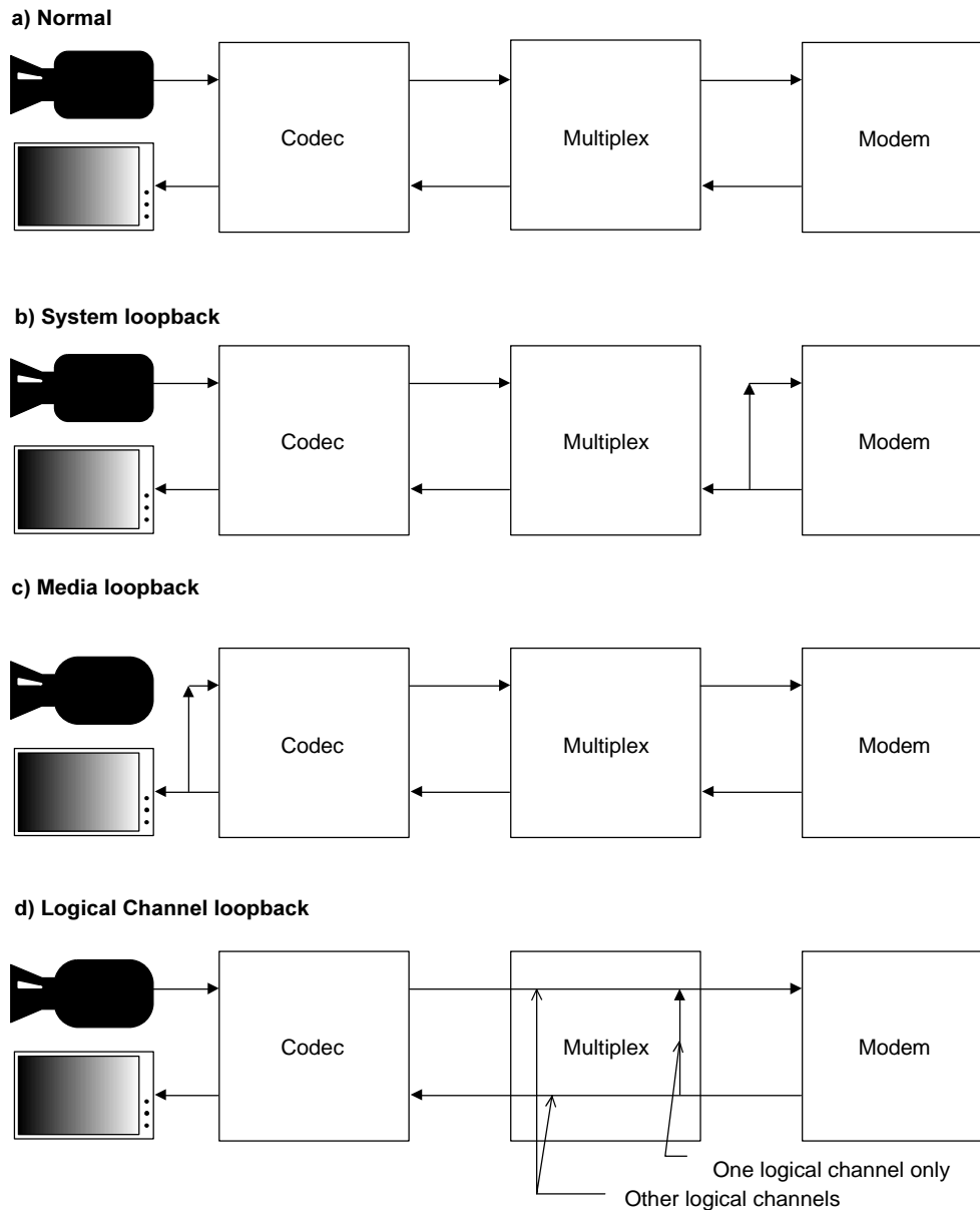
FIGURE 5/H.324
