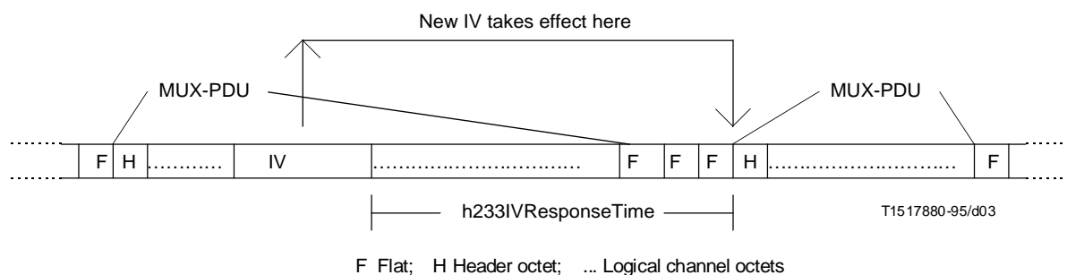
FIGURE 3/H.324
