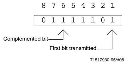
FIGURE B.1/H.324
